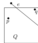
Figure 1 The points p and q are separated in Q by the edge e .
