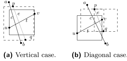
■ Figure 3 Examples where edge e is a nearer to v than c .
