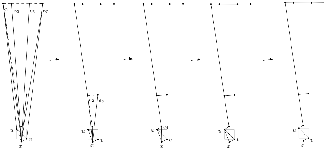
■ Figure 4 Example of a sequence with a spanning tree of a 10-point set that converges in 4 steps. The dashed edges represent the appearing edges at stage i + 1 .
