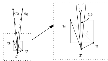
■ Figure 5 The dashed edges have length \|e\|_\infty = \frac{2\ell}{3^{i-1}} and all the xa -paths different from (x, a) contain one of the endpoint different from x of e_2 or e_6 .
