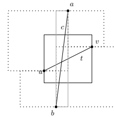
■ Figure 2 The dotted squares represent Q(a, v) , Q(b, v) , Q(a, u) and Q(b, u) , which have shorter weight than \|ab\|_\infty = h(a, b) .
